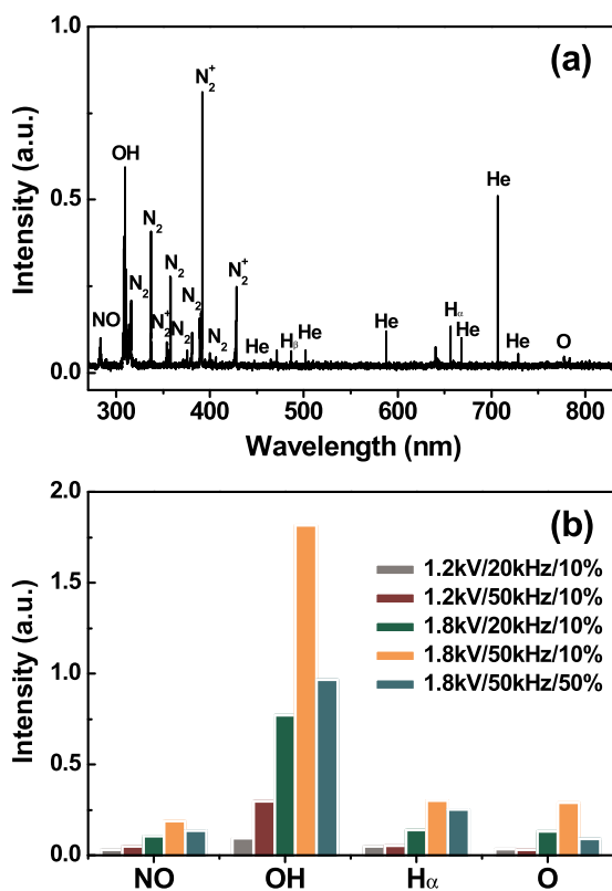
FIG. 5. (a) Emission spectra from observed in the helium/oxygen plasma for the pulsed dc-driven source (1.6 kV, 50 kHz, 10%, 500 sccm). (b) Comparison of the emission intensities from NO_x , OH, H_x , O radicals for different operating conditions.
