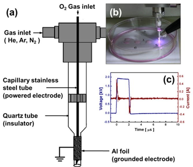
FIG. 1. (a) Schematic presentation of the jet device, (b) photograph of the plasma-cell interaction, and (c) waveforms of applied voltage and total current.
